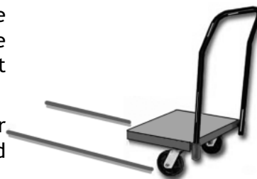
Figure 4. Tricycle-gear airplane comparison. With the mass ahead of the main wheels (this comparison has a person pulling the hand cart), the tricycle-gear airplane tracks straight during takeoff.
